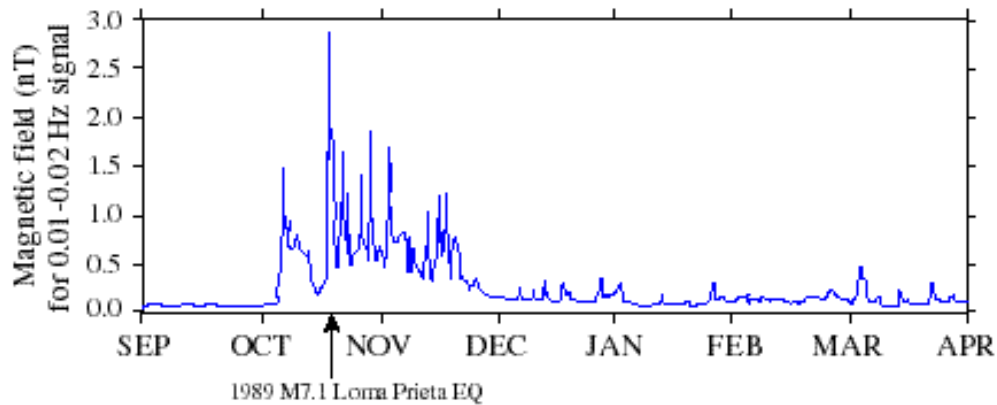
Figure 1 Magnetic field activity at Cormilito, CA (COR on Figure 3) from 9/89 – 4/90. Note increase in activity two weeks prior to the main shock, much larger amplitudes starting three hours before the main shock (Fraser-Smith et al., 1993) and the continuing high fields for over a month following the main shock (Fenoglio et al., 1993).
