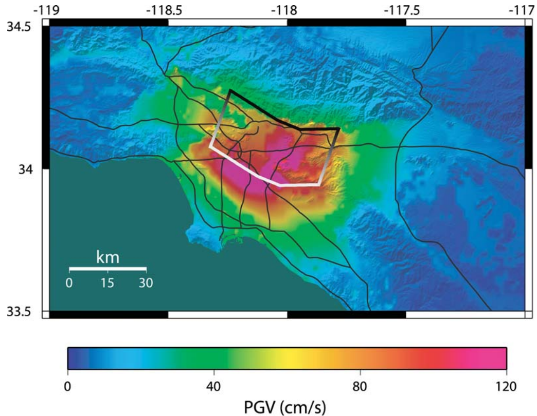
Peak ground velocity (PGV) map for a postulated magnitude 7.4 earthquake on Puente Hills fault in Los Angeles, California
