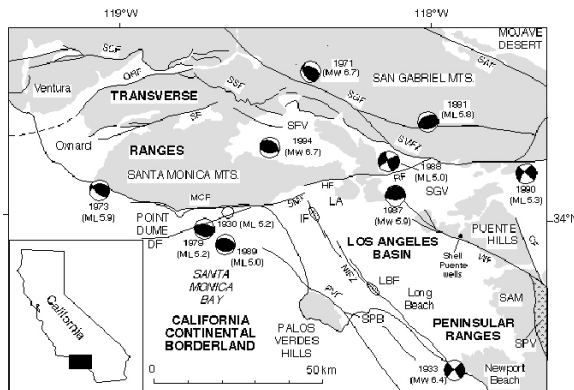
Fig. 1: Index map showing the triple join between the Whittier, Chino, and Elsinore faults and a possible join between the Santa Monica, Dume, and Palos Verdes faults. The 1979 and 1989 earthquakes in Santa Monica Bay do not fit the existing fault models.
